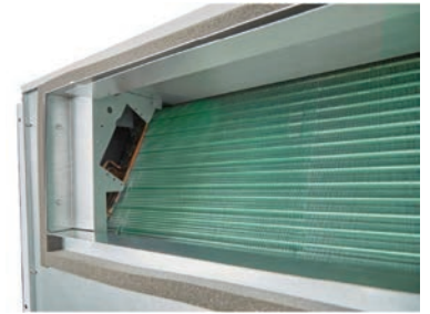
Hydrophilic Green Coil (standard)
